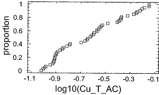
Quantile Plot
